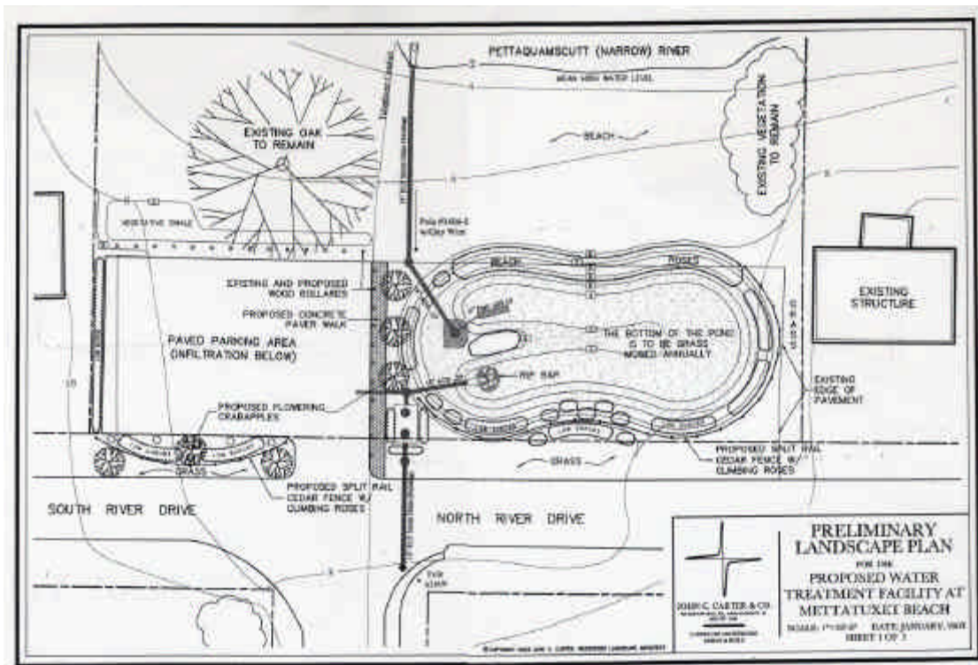
SRICD developed the design and engineering for the storm water treatment system, while John Carter of Narragansett produced a landscape plan.
